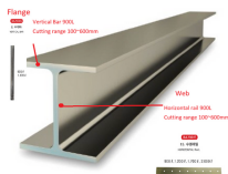
BA 290 H-beam Cutting Range
